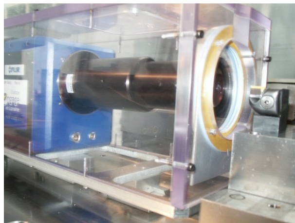
Figure 2 - Experimental setup
