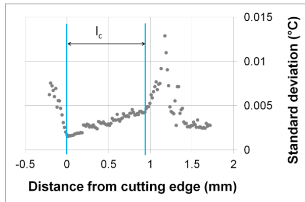
Figure 12 - Example of contact length determination through standard deviation analysis (V_c = 150 \text{ m/min}, f = 0.3 \text{ mm/rev}, a_p = 2 \text{ mm})
