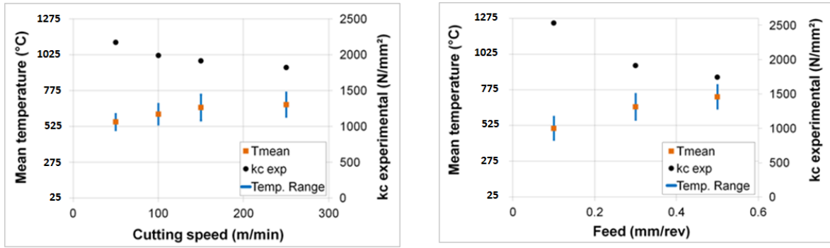
(a) f = 0.3 \text{ mm/rev} - a_p = 2 \text{ mm} (b) V_c = 150 \text{ m/min} - a_p = 2 \text{ mm} Figure 16 - Mean temperature evolution with cutting speed (a) and with feed (b).
