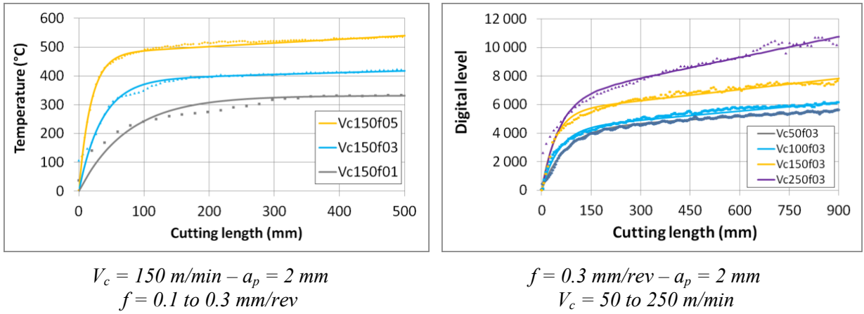
Figure 14 - Temperature evolution function of cutting length
