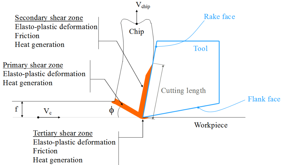
Figure 1 - Heat sources in the orthogonal cutting process
