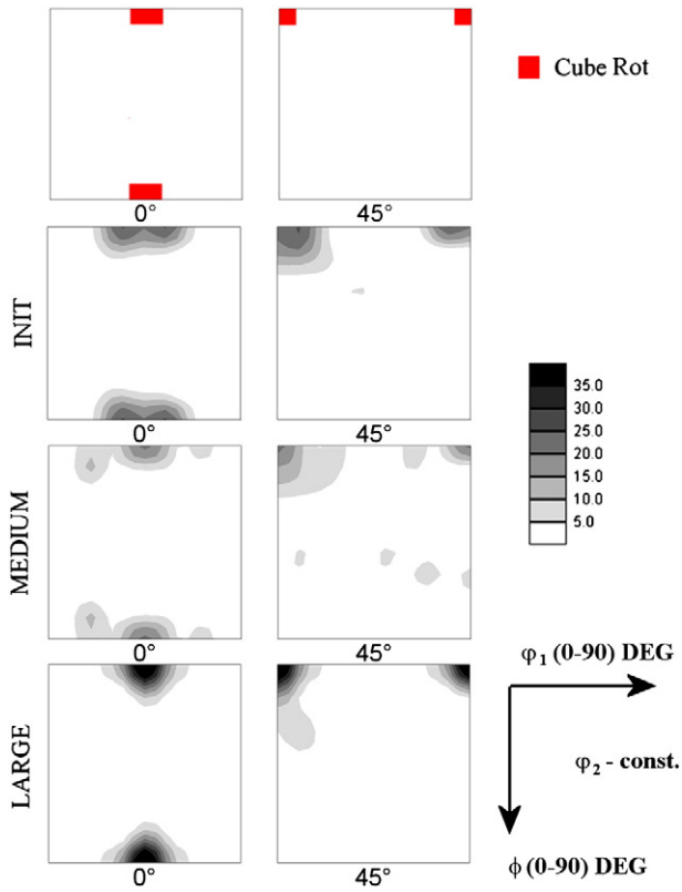
Fig. 10 – Experimental textures for various degrees of deformation for the alpha phase—ODF sections ( \varphi_2=0^\circ, 45^\circ ).
