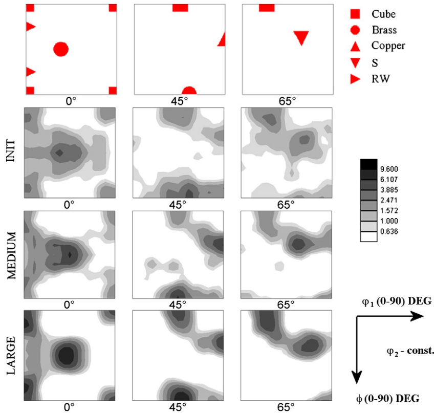
Fig. 11 – Experimental textures for various degrees of deformation for the gamma phase—ODF sections ( \varphi_2=0^\circ, 45^\circ and 65^\circ ).
