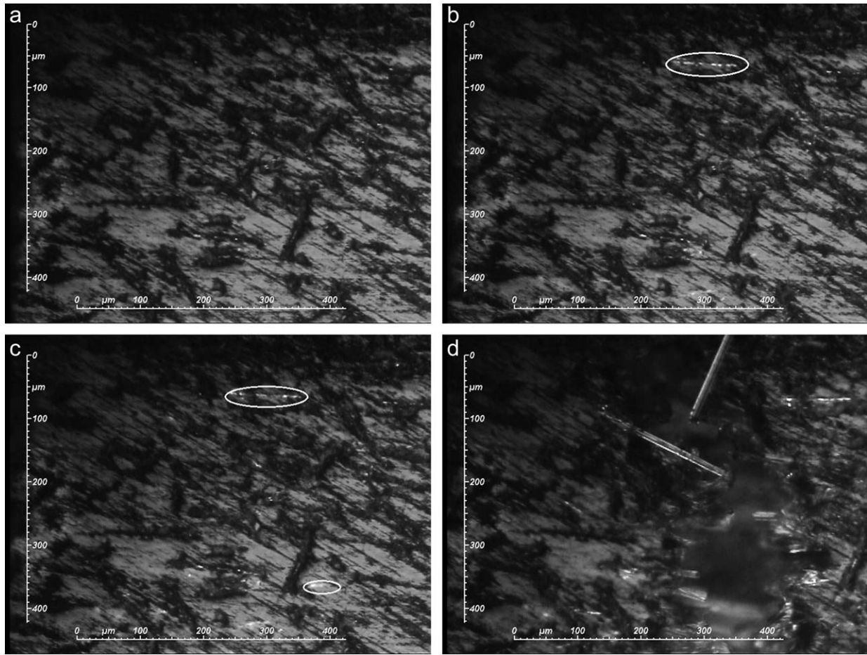
Figure 6 Optical microscopy observation of the most constrained part of a specimen tested at 10 Hz and \epsilon = 0.017 (poly-sequential test) (a) initial, (b) 30,000 cycles, T = 57^\circ\text{C} , (c) 45,000 cycles, T = 60^\circ\text{C} , (d) 60,000 cycles, T = 62^\circ\text{C} .
