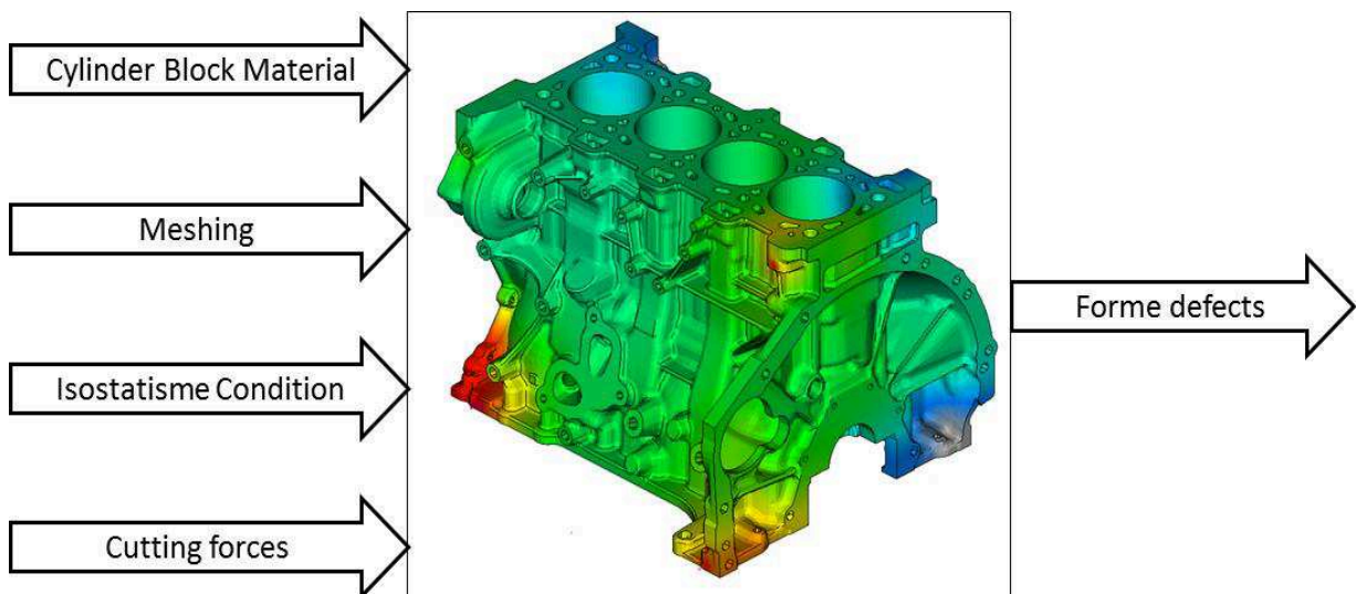
(Fig.3: Rough line boring FEM tool- Calculation Methodology)
