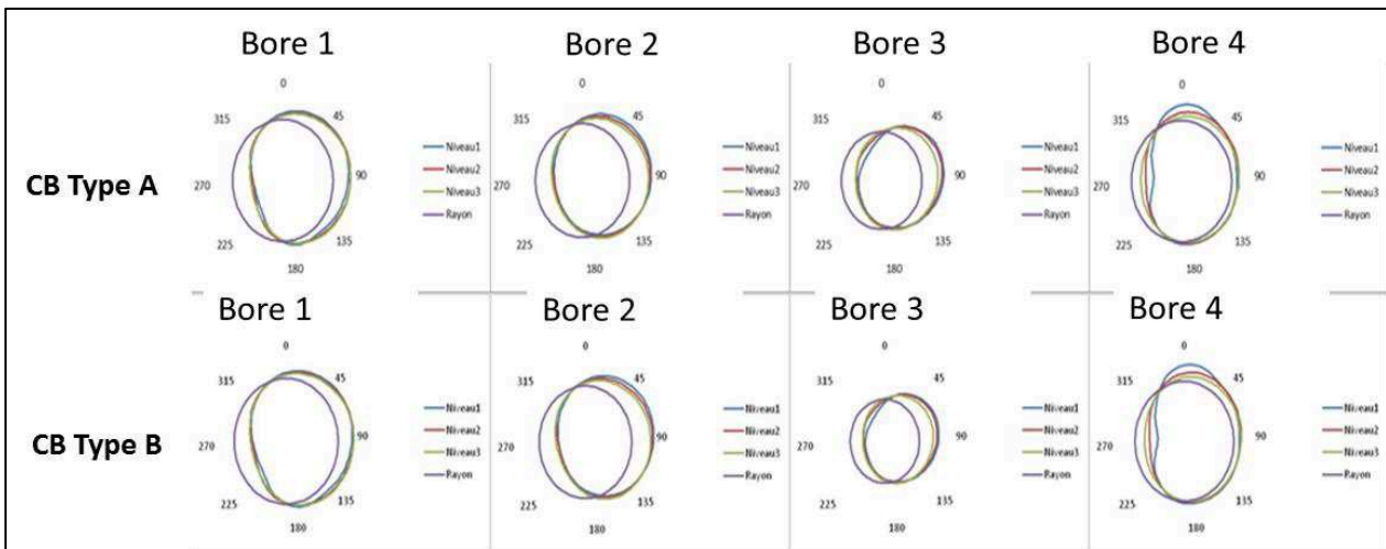
(Fig.9: Bore distortion comparison between type A and B cylinder blocks under cutting and clamping forces)
