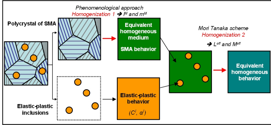
Figure 3: Homogenization strategy leading from SMA polycrystalline matrix with spherical elastoplastic inclusions to equivalent homogeneous medium (Piotrowski, 2010)
