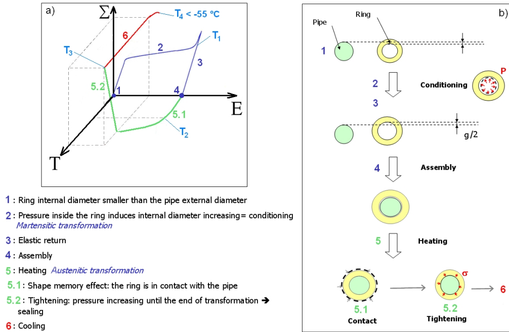
Figure 2: Applied thermo-mechanical cycle on a shape memory ring - a) Stress ( \Sigma ) - strain ( E ) - temperature ( T ) diagram - b) Corresponding tightening steps ( g is the clearance between internal diameter of the SMA ring and the external one of the tube after elastic return)
