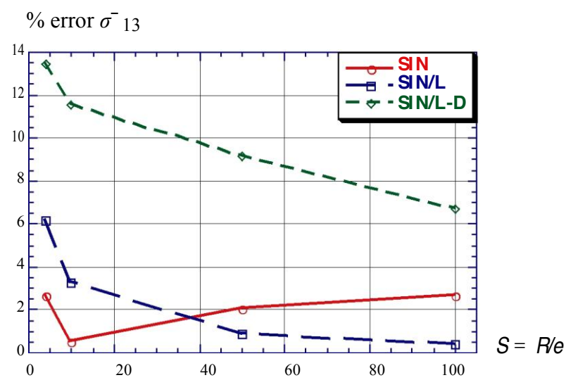
Fig. 11. Homogeneous case ; ratio R/a = 3/\pi ( R/a \sim 1 ). Comparisons between SIN, SIN/L, SIN/L-D models.
