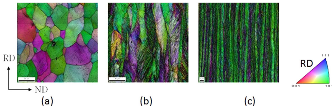
Fig. 11. EBSD maps measured on the transverse section of the cold-rolled material after (a) 15%, (b) 61% and (c) 88% rolling strains. Maps of 100 \mu\text{m} \times 100 \mu\text{m} , step size of 0.2 \mu\text{m} .
