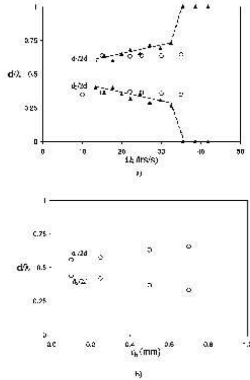
FIG. 12. Evolution of the distances between two consecutive bubble rings: (a) with the inner cylinder rotational velocity \Omega_{c1} , for a 1 mm bubble. \blacktriangle - \blacktriangle - \blacktriangle experimental observed distances and \circ - \circ - \circ - \circ computed values ( C_1=0.5 ); (b) with bubble radius, for Re/Re_{c1}=4.8 (computed values with C_1=0.5 ).
