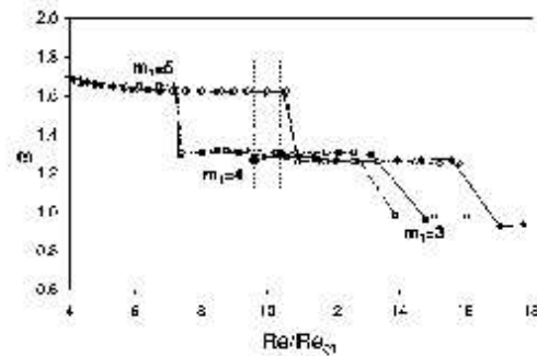
FIG. 8. Evolution of the azimuthal wave dimensionless frequency and the wave number vs Reynolds number (repeatability is investigated: solid and dashed line) \diamond-\diamond-\diamond-\diamond and \circ-\circ-\circ-\circ : single phase flow. \blacksquare-\blacksquare-\blacksquare-\blacksquare and \square-\square-\square-\square : first procedure, near cavitation inception, for a fixed vacuum tank pressure ( Pe=2700 Pa), by decreasing Reynolds number. \bullet-\bullet-\bullet-\bullet : other procedure, at cavitation inception, for different fixed Reynolds numbers, by decreasing Pe .
