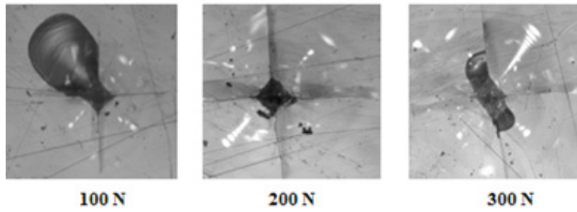
Float glass : Scale 400 μm
