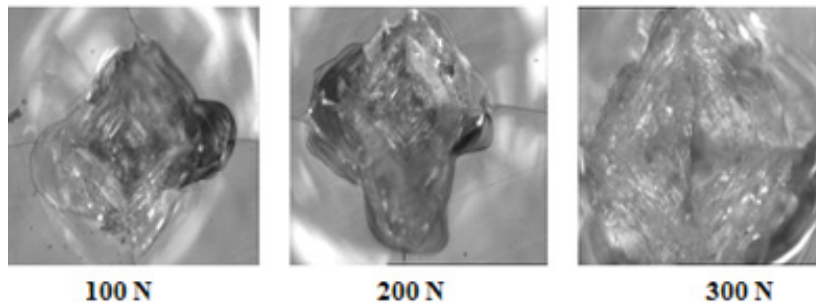
Crown K5 glass : Scale 500 μm
