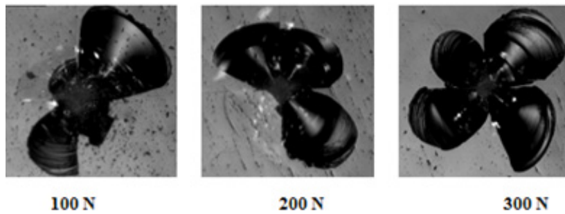
Heavy flint glass : Scale 500 μm
