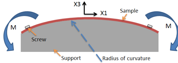
Figure 3: Side view of the support-sample assembly. Bending moment is applied to the sample resulting in a constant uniaxial stress.
