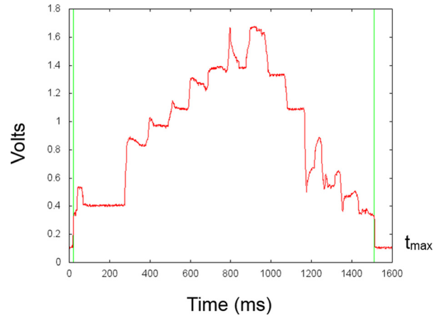
Fig. 12 Typical pressure sensor signal reflecting a stepwise pressure increase and pressure decrease as applied qualitatively by the user
