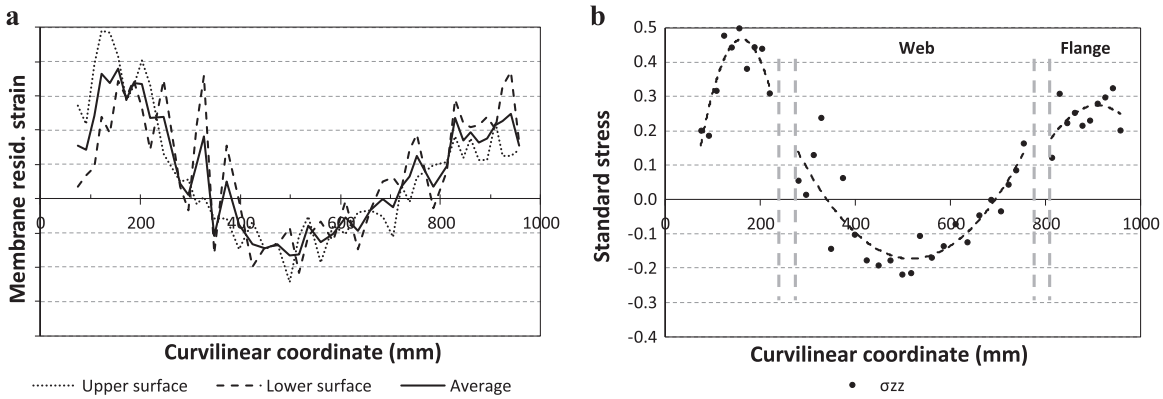
Fig. 13. (a) Membrane strain on the two surfaces & average strain in the sheet pile 2: after cooling, in the longitudinal direction, (b) normalised longitudinal residual stress in the sheet pile 2: after cooling, in the longitudinal direction.
