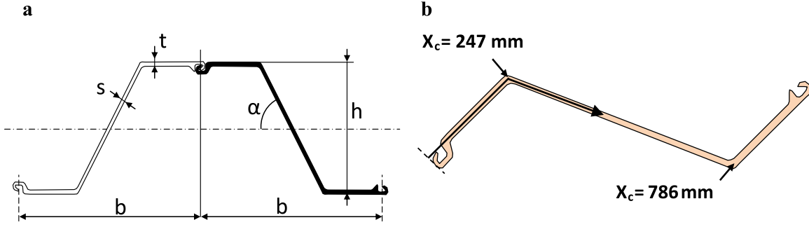
Fig. 2. (a) Sheet pile geometry (AZ 38-700+1, b=700 mm, h=501 mm, t=19 mm, s=14.2 mm, \alpha=63.2^\circ , length=6000 mm), (b) location of curvilinear coordinates: X_c .
