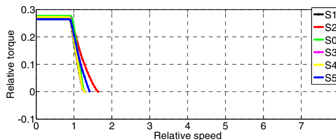
Figure 9: torque/speed characteristic in fault mode (2 adjacent phases opened)
