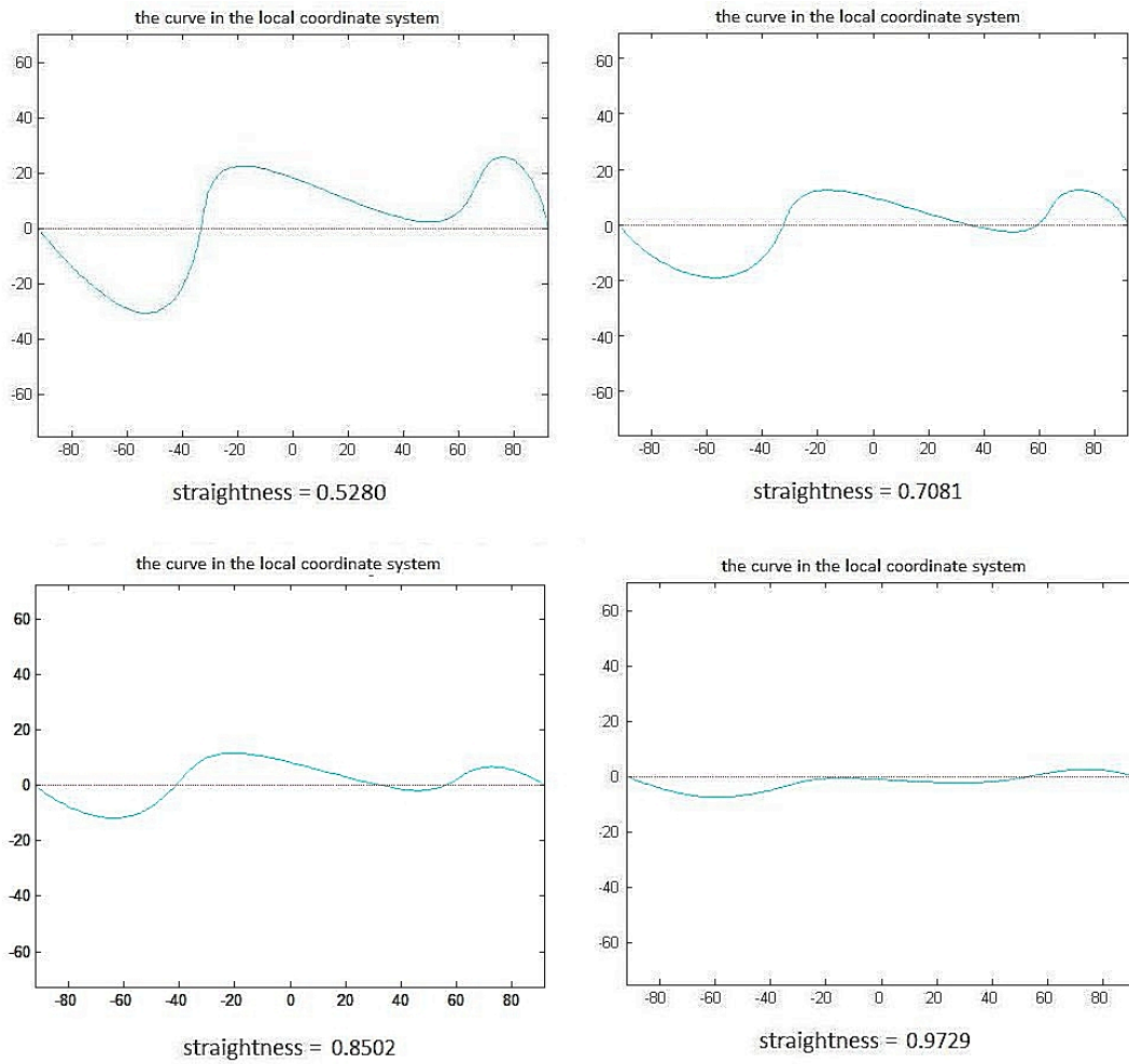
Fig. 4: Some examples of straightness evaluation.
