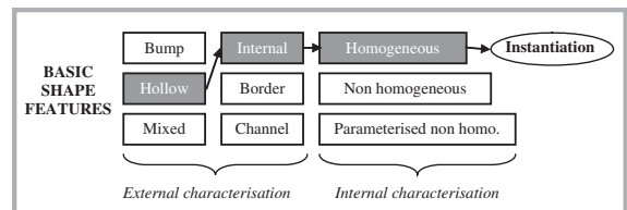
Fig. 5. BSF sub-classifications using internal and external properties.
