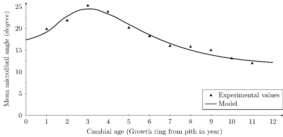
Fig. 2. Variation in MFA with cambial age for seven poplar clones at breast height (measurements from Fang et al. (2006))
