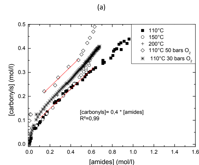
Fig. 7. Correlation between oxidation products formation for (a) DGEBA/IPDA and (b) DGEBA/TTDA.
