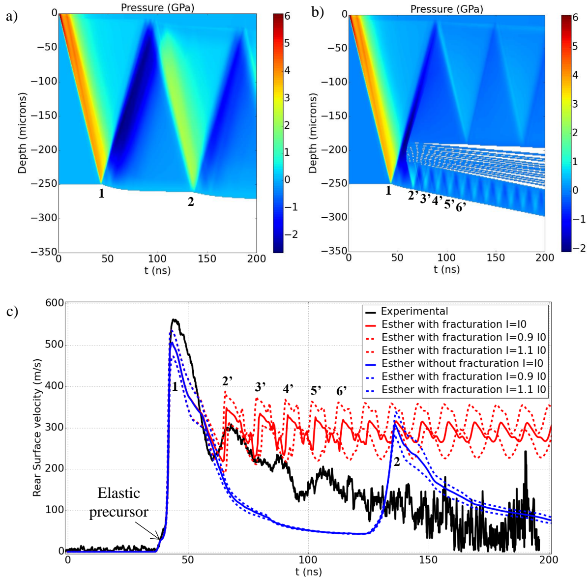
Fig. 3 Space-time diagram without fracturation model (a), with fracturation model (b) and rear surface velocity profile (c) obtained by simulation ( \pm 10\% on E ) with fracturation (red), without fracturation (blue), and compared to the experimental signal – Pure Aluminum – E=18.3 \text{ J} – t=250 \text{ }\mu\text{m} – \tau=10 \text{ ns} – \text{dfoc}=1 \text{ mm} ( I=170 \text{ GW/cm}^2 ) Typically, rear free surface velocity is characterized by successive oscillations corresponding to shock waves going back and forth within the target [14]. The period of these oscillations is given by equation (1).
