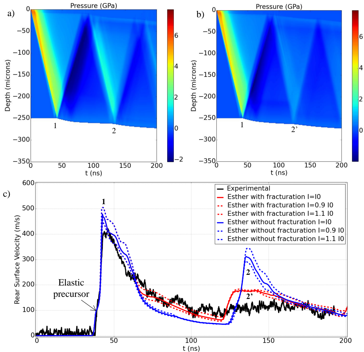
Fig. 4 Space-time diagram without fracturation model (a), with fracturation model (b) and rear surface velocity profile (c) obtained by simulation ( \pm 10\% on E) with fracturation (red), without fracturation (blue), and compared to the experimental signal – Aluminum 6061 – E=20.3 \text{ J} – t=250 \text{ }\mu\text{m} – \tau=10 \text{ ns} – d_{\text{foc}}=1 \text{ mm} ( I=180 \text{ GW/cm}^2 )
