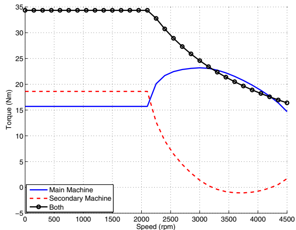
(a) Torque vs speed
