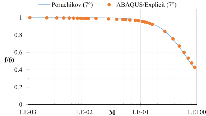
Fig. A.1. Evolution of the slamming coefficient with the Mach number in the case of the impact of a cone with a deadrise angle of 7^\circ on pure water ( f_0 is the value of the slamming coefficient for M tending towards zero). Comparison between the analytical model of Poruchikov (1973) and ABAQUS/explicit simulations.
