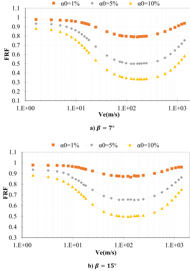
Fig. 8. Force reduction factor F_\alpha/F_0 (from ABAQUS/Explicit simulations) as a function of the expansion velocity V_e for three void fractions \alpha_0=1\% , \alpha_0=5\% and \alpha_0=10\% . a) deadrise angle \beta=7^\circ , b) deadrise angle \beta=15^\circ .
