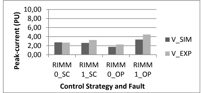
Fig. 20: RIMM's peak current in degraded mode for different control strategies in simulation and experimentally.
