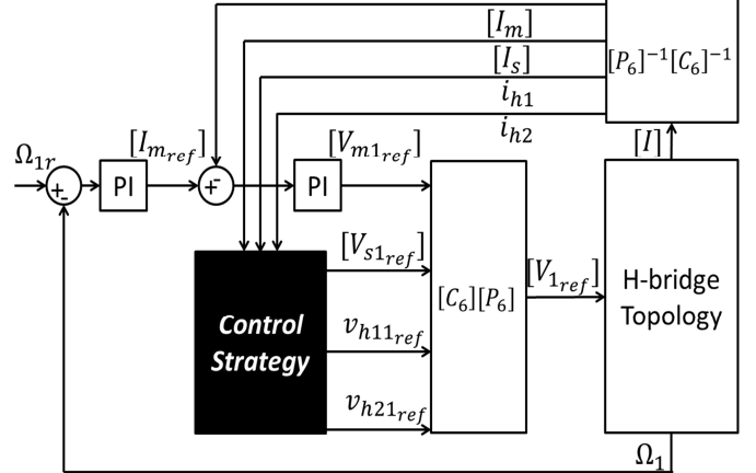
Fig. 8: Control diagram of one machine in H-bridge topology.
