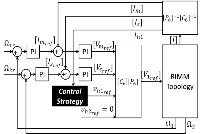
Fig. 7: Control diagram of RIMM topology.
