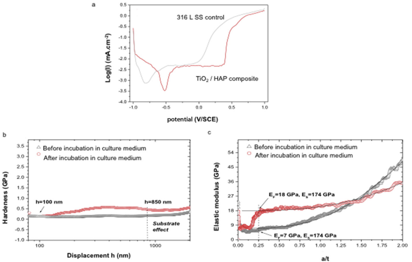
Fig. 5. Corrosion and mechanical features. (a) Potentiodynamic curves of \text{TiO}_2/\text{HAP} composite (red line) and 316 L SS (black line) after 7 days of culture medium soaking. (b–c) Indentation data versus the indenter displacement applied on the \text{TiO}_2/\text{HAP} composite coating for the determination of the (b) hardness and (c) elastic modulus before (black line) and after (red line) 7 days of culture medium soaking.
