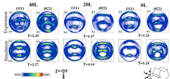
Fig. 33. Experimental and simulated orientation distribution functions for machining of copper [31].
