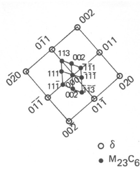
Fig. 4. Decomposition of \delta ferrite after aging at 550 °C during 1000 h (TEM examination): (a) F.K phase (I phase) and M_{23}C_6 carbide at the \delta/\gamma interface; (b) SAD of F.K phase and \delta ferrite matrix; (c) SAD of M_{23}C_6 carbide and \delta ferrite matrix.
