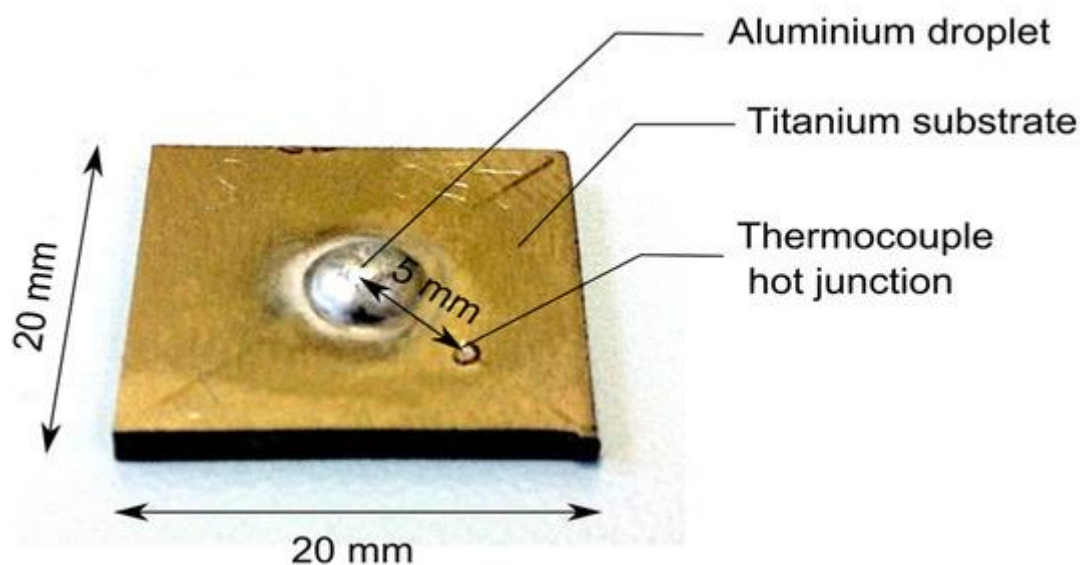
Figure 7. Experimental configuration.
