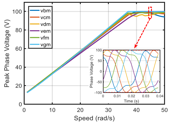
Fig. 7. Voltage-speed characteristics and instantaneous phase voltage at 45 rad/s over the base speed (37 rad/s) when phase a is open-circuited with strategy 1.
