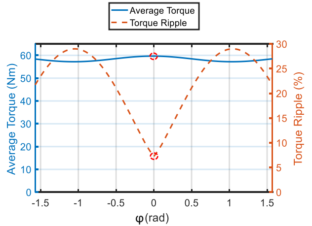
Fig. 4. Impact of \varphi = \varphi_3 on the average torque and torque ripple when phase a is open-circuited.
