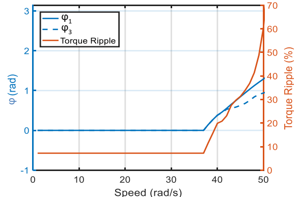
Fig. 9. Initial phases ( \varphi_1, \varphi_3 ) and torque ripple when phase a is open-circuited with strategy 1.
