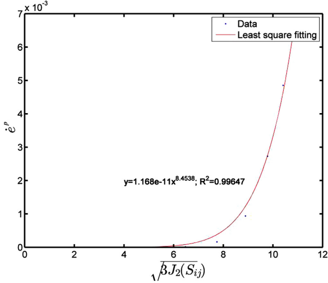
Fig. 1. A fitting result of \dot{\epsilon}^p vs. \sqrt{3}J_2(\dot{S}_{ij}) , under 343 number of grains; P_r^{app} is 1.168e-11 and the corresponding values of n^{app} and K^{app} are 7.45 and 29.29, respectively.
