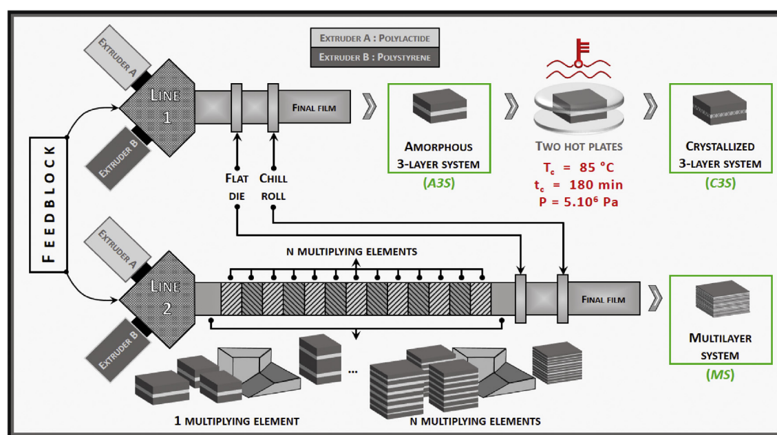
Fig. 1. Principle of the layer multiplying co-extrusion process.
