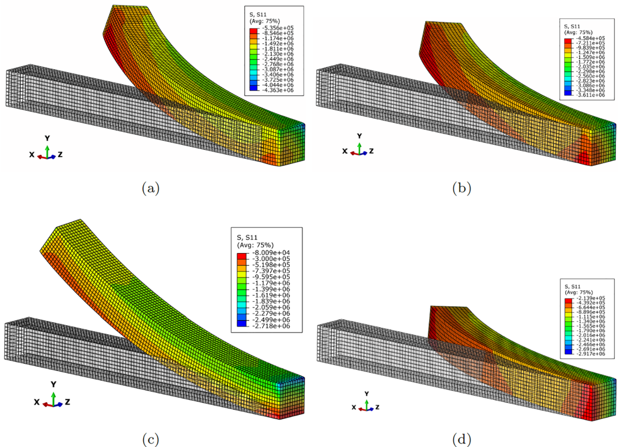
Fig 3. Different configurations of the finger segment. (a) F_1 = 100\text{N}, F_2 = 100\text{N} ; (b) F_1 = 50\text{N}, F_2 = 100\text{N} ; (c) F_1 = 100\text{N}, F_2 = 0\text{N} ; (d) F_1 = 10\text{N}, F_2 = 100\text{N} . The legend corresponds to S_{11} , the first component of the second Piola-Kirchhoff stress tensor. Symmetric configurations can be obtained by actuating the tendons situated at opposite positions.
