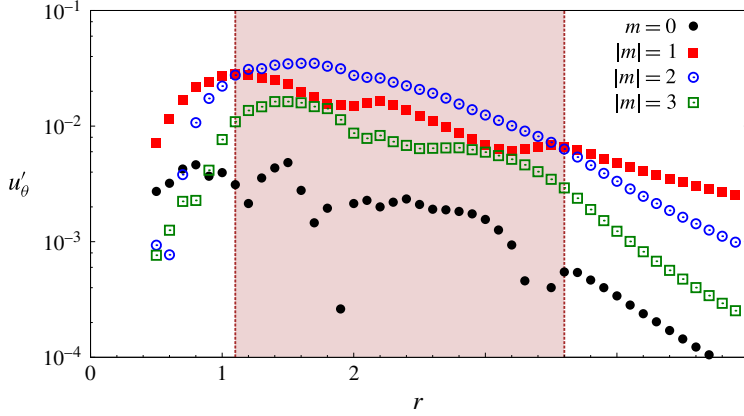
FIGURE 6. (Colour online) Results for Re = 5000 isolated vortex: Fourier decomposition of the azimuthal component of the T = 4.8 , E(0) = 3 \times 10^{-3} nonlinear optimal perturbation ( t=0 ) velocity field at various radial locations. Here m is the azimuthal wavenumber. The shaded part corresponds to the radial segment between the two spiral dislocations in the nonlinear optimal perturbation shown in figure 5(c).
