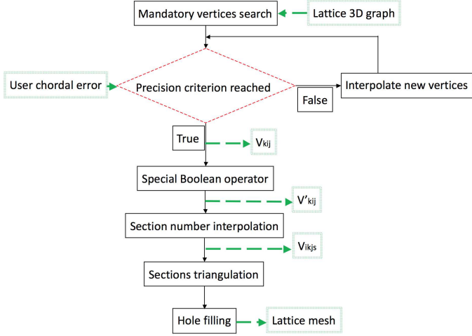
Figure 7: Overall framework of the LSLT technique
