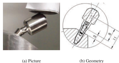
Fig. 1. Implant internal threaded connection on abutment [2]
