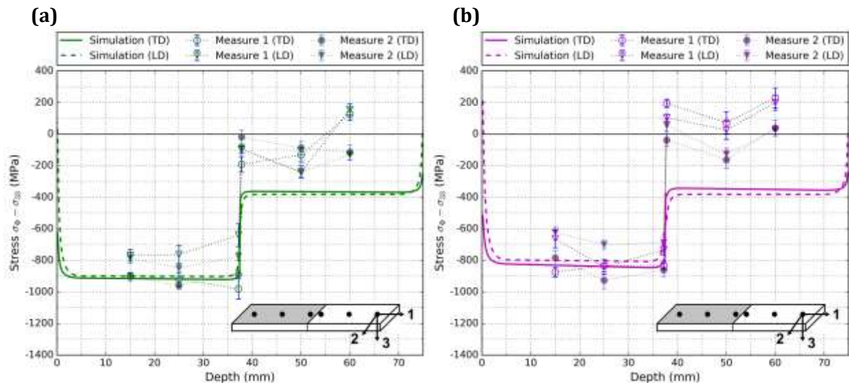
Fig. 2: residual stresses distributions along the longitudinal direction (4 μm depth) for samples of 5 mm thickness: a) partially shot-peened SP1, b) and partially shot-peened SP2
