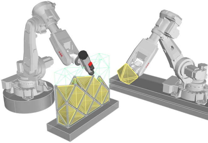
Fig. 1. Printing mortar while assembling blocks.
