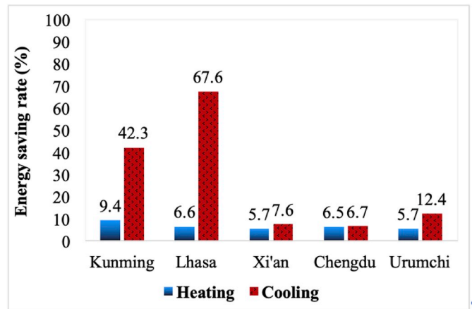
Fig. 2. Heating and cooling energy saving rate in different Chinese cities (modified from Ref. [18]). Copyright (2019), with permission from Elsevier.
