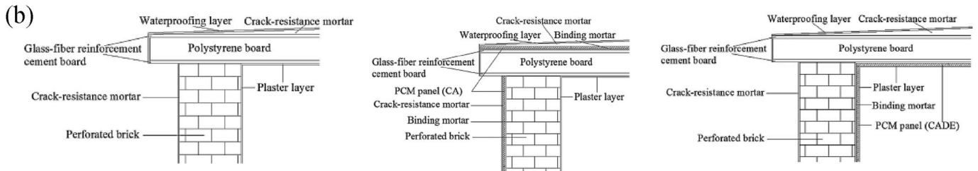
Fig. 16. (a) Test room, sections of the wall structure of the (b) Conventional test cell, (c) PCMIW, and (d) PCMIW [124]. Copyright (2019), with permission from Elsevier.
