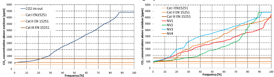
Figure 3: Frequency distribution of the measured CO 2 concentration above outdoor for the whole occupied period (on the left) and for each ventilation strategy during the occupied period (on the right)
