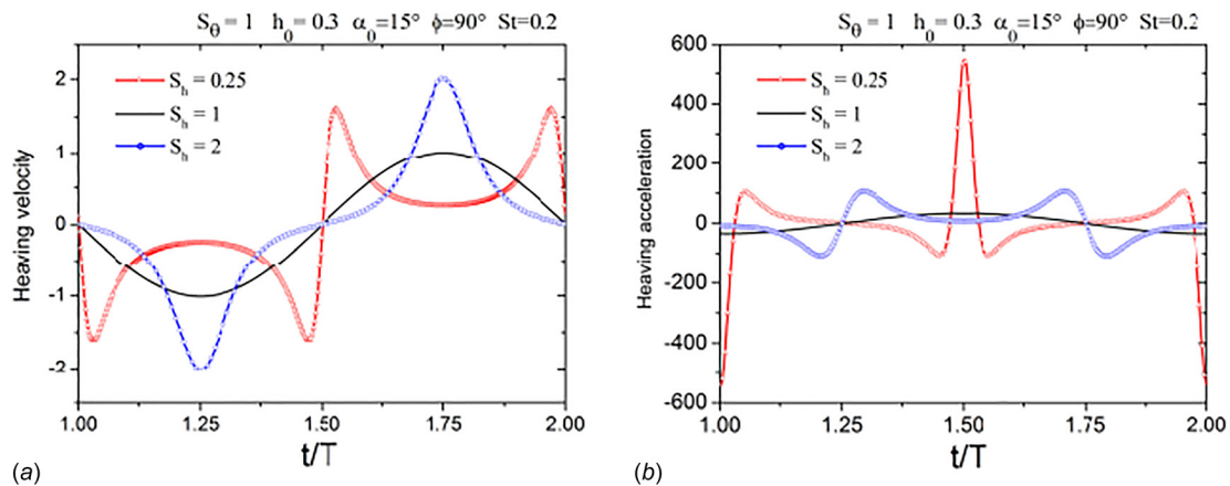
Fig. 23 (a) velocity and (b) acceleration of the foil during one flapping cycle for S_h = 0.25 , S_h = 1 and S_h = 2
