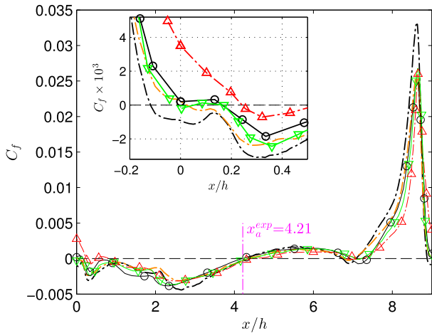
Fig. 12 Friction coefficient along the bottom wall at Re=10595 ; -\cdot-\cdot- 512 \times 256 \times 256 ( M = 0.2 ); -\cdot-\cdot- 512 \times 256 \times 256 ( M = 0.1 ); -\cdot\Delta\cdot LES of Ziefle et al. [19]; -\circ- LES of Xia et al. [18]; -\nabla- LES of Diosady et al. [61]
