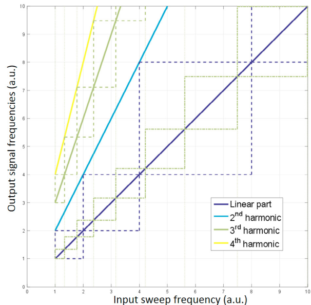
Fig. 2. Input sweep frequency versus output signal frequencies for a 4 th order PHM and windowing choices examples (no overlap): linear part [optimal] (blue dashed lines), third harmonic [optimal] (green dashed lines), linear part [suboptimal] (green dot-dashed line).
