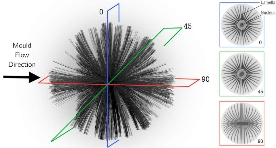
Fig. 14. Oriented spherulitic structure induced by the injection molding.
