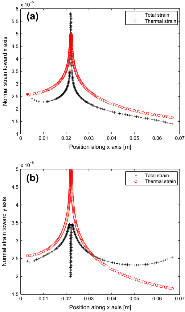
Fig. 12. Total and thermal normal strain distribution along x axis in the case of E4 test ( \Delta K = 20 \text{ MPa } \sqrt{\text{m}} ; R = 0.1 ): (a) normal strain toward x axis, (b) normal strain toward y axis.
