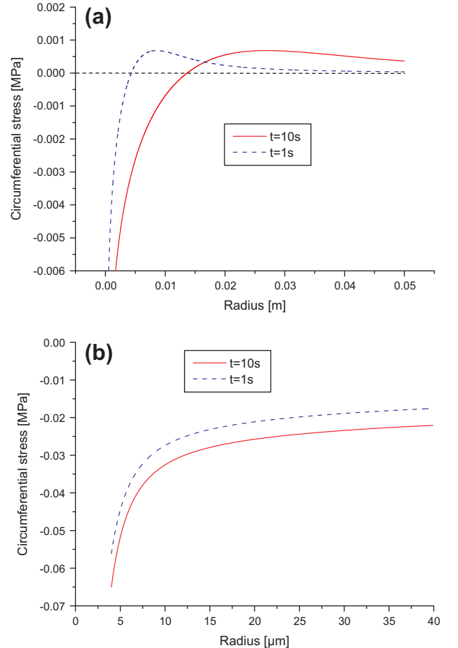
Fig. 2. The circumferential stress distribution at various times for a unit heat source q = 1 \text{ W m}^{-1} and r_R = 4 \text{ }\mu\text{m} : (a) general view, (b) enlargement near the reverse cyclic plastic zone, from [6].
