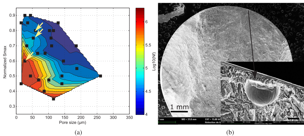
Fig. 17. (a) Generalized Kitagawa-Takahashi map for 45^\circ batches showing the effect of spherical gas pores (indicated by arrows) and (b) SEM images of crack initiation from a spherical gas pore.
