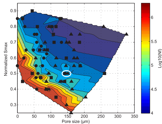
Fig. 18. S-\sqrt{area}-N_f map for only surface lack-of-fusion pores (i.e. without internal pores and spherical gas pores); circular dots = 0^\circ specimens, square dots = 45^\circ specimens, triangle dots = 90^\circ specimens.
