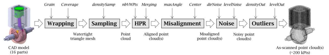
Figure 3: Virtual Reverse Engineering modular framework generating as-scanned point clouds from CAD assembly models.
