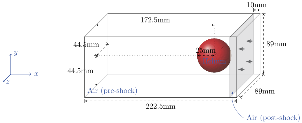
Fig. 5. Sketch of the initial configuration for the shock–bubble interaction TC1. The computational domain is [247.5, 470] \times [0, 89] \times [0, 89] mm 3 .
