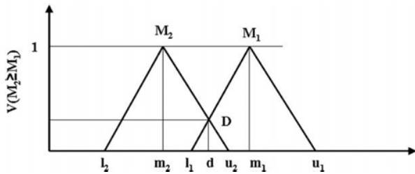
FIGURE 5. The intersection between M_1 and M_2 .
