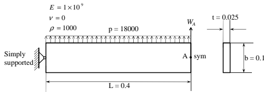
Fig. 12. Simply supported elastic beam
