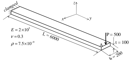
Fig. 10. Elastic cantilever beam under impulsively-applied loading
