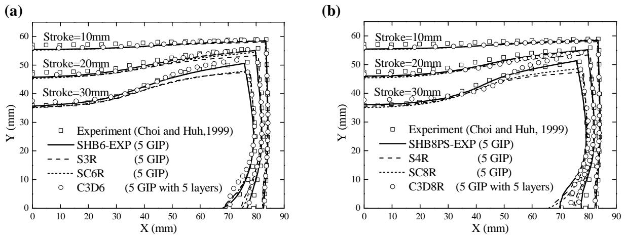
Figure 31. Prediction of flange contours at different punch strokes: comparison between the SHB-EXP simulation results using 5 through-thickness GIP, ABAQUS element results, and experimental measurements; (a) triangular shell / prismatic elements, and (b) quadrilateral shell / hexahedral elements
