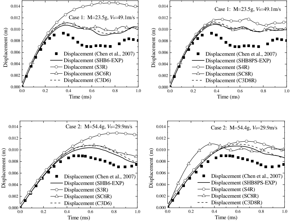
Figure 20. Displacement history at the plate center, obtained with the SHB-EXP and ABAQUS elements along with the reference solutions (Chen et al., 2007), for case 1 (top) and case 2 (bottom)
