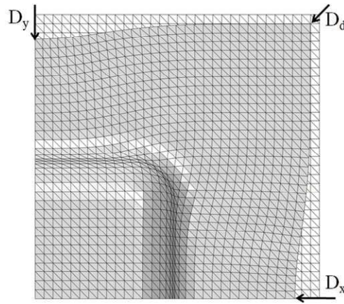
Figure 26. Illustration of the draw-in distances of the square cup after forming
