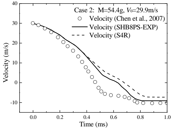
Figure 15. History of velocity (left) and impact force (right) for the projectile, obtained with the SHB-EXP and ABAQUS shell elements along with the reference solutions for case 2
