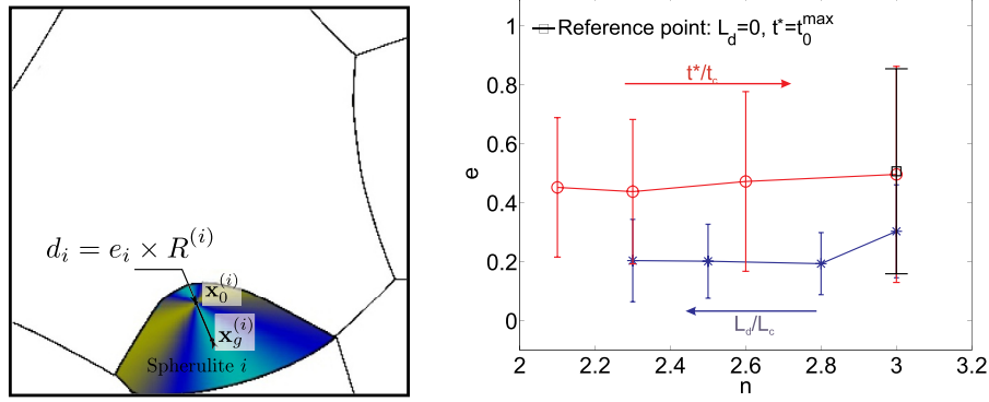
Fig. 10. a) Schematic representation of the algorithm used to generate the microstructure under periodic boundary conditions. b) e versus Avrami parameter n for the two algorithms which introduce nucleation saturation. L_c = 21.5 \mu\text{m} , t_c = 2.15 \times 10^3 \text{ s} . The red curve denotes the effective nucleation time algorithm, and the blue curve denotes the nucleation excluded zone algorithm. (For interpretation of the references to color in this figure legend, the reader is referred to the Web version of this article.)
