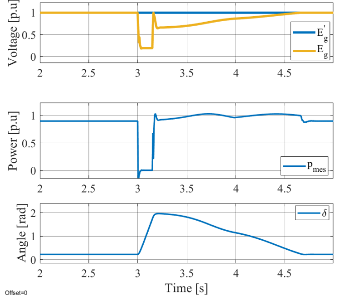
Offset=0 Fig. 9. Dynamic behavior of the system subjected to a three phase bolted fault.
